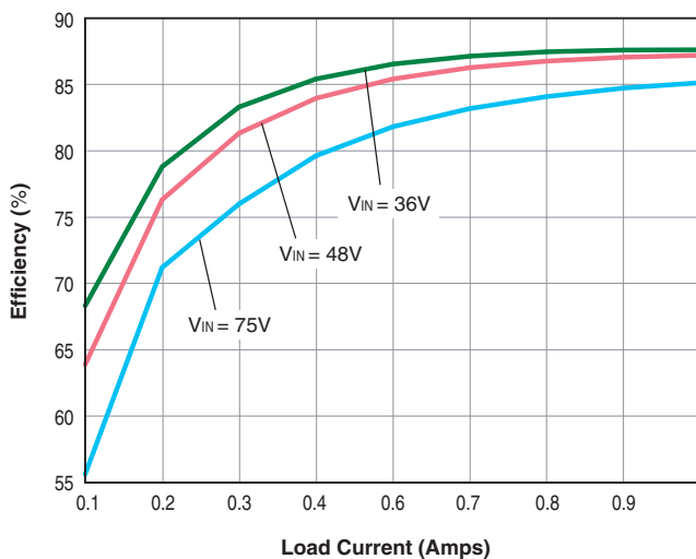
UWR-15/1000-D48A Efficiency vs. Line and Load
